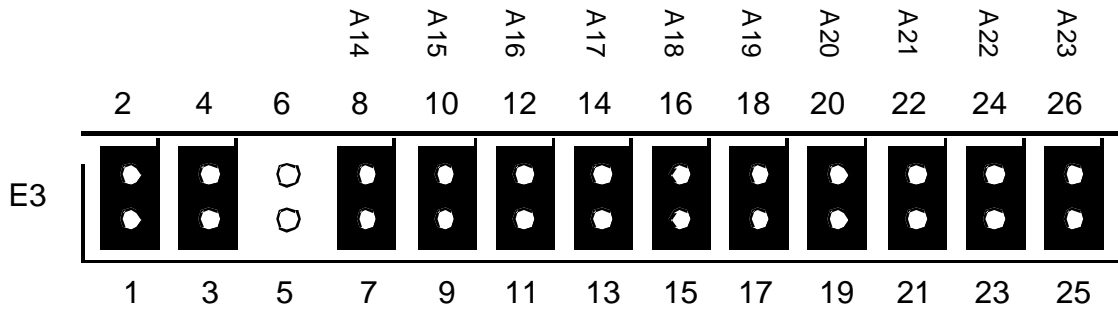
Figure 2-4: Board Configuration Jumpers
