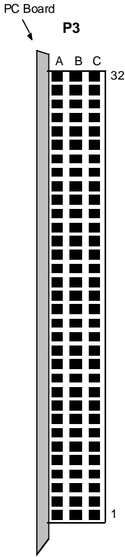
Figure 2-7: P3 Connector
