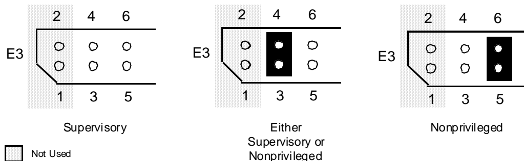
Figure 2-2: Supervisory and Nonprivileged Access Modes and Jumper Locations
