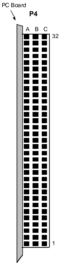
Figure 2-8: P4 Connector
